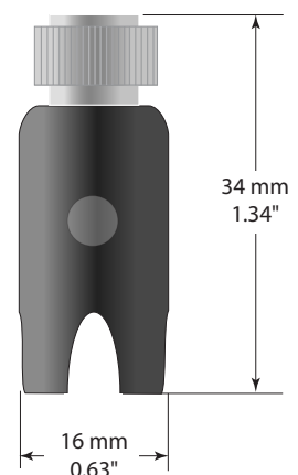
TT-MINI-PROBE dimensions
